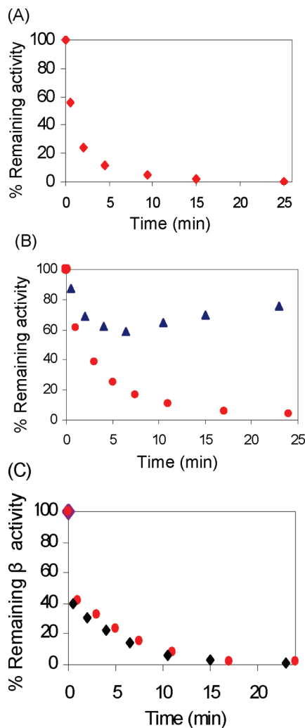
FIGURE 1: Time-dependent inactivation of E. coli wt-RNR (3 \mu M) or C225S-RNR by F_2 CDP (3 or 6 \mu M) in the absence of reductant, assayed by method 1 or method 2. (A) Method 1: inactivation mixture diluted 10-fold with 1 F_2 CDP/ \alpha 2 . (B) \alpha (blue \blacktriangle ) and \beta (red \bullet ) inactivation mixture diluted 20-fold in the presence of a 5-fold excess of the second subunit. (C) Method 2: as in (B) except C225S-RNR replaced wt-RNR. The remaining \beta activity was assayed in the absence of reductant (red \bullet ) and in the presence of reductant (DTT, black \blacklozenge ).
