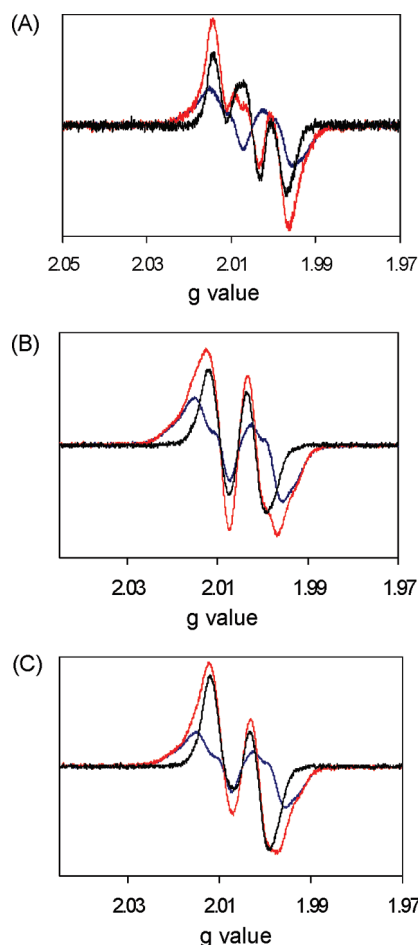
FIGURE 5: EPR spectrum at 9 GHz of E. coli wt-RNR ( 15\ \mu M ) or C225S-RNR ( 15\ \mu M ) inactivated by F_2CDP or [1'-^2H]-F_2CDP . (A) The reaction mixture with F_2CDP was frozen in liquid N_2 at 45 s (red) and is a composite of Y\cdot and new radical. The Y\cdot (blue) was subtracted from the red spectrum to give the black spectrum of the new radical. (B) As in (A) except that [1'-^2H]-F_2CDP replaced F_2CDP . (C) As in (A) except that C225S-RNR and [1'-^2H]-F_2CDP replaced wt-RNR and F_2CDP .
