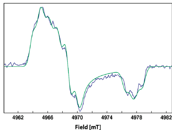
FIGURE 3: Echo-detected 139.5 GHz EPR spectrum of F_2 CDP-inactivated RNR recorded at 65 K. 1000 shots were accumulated for each point in the spectrum. The stimulated echo pulse width was t_{\pi/2} = 56 ns and t_p = 200 ns. g -values obtained from the spectrum are as follows: g_x = 2.00738 , g_y = 2.00592 , and g_z = 2.00230 . Two hyperfine couplings were used in the simulation with A_1 = (11.4, 14.6, 12.8) and A_2 = (8.5, 8.5, 8.5) .
